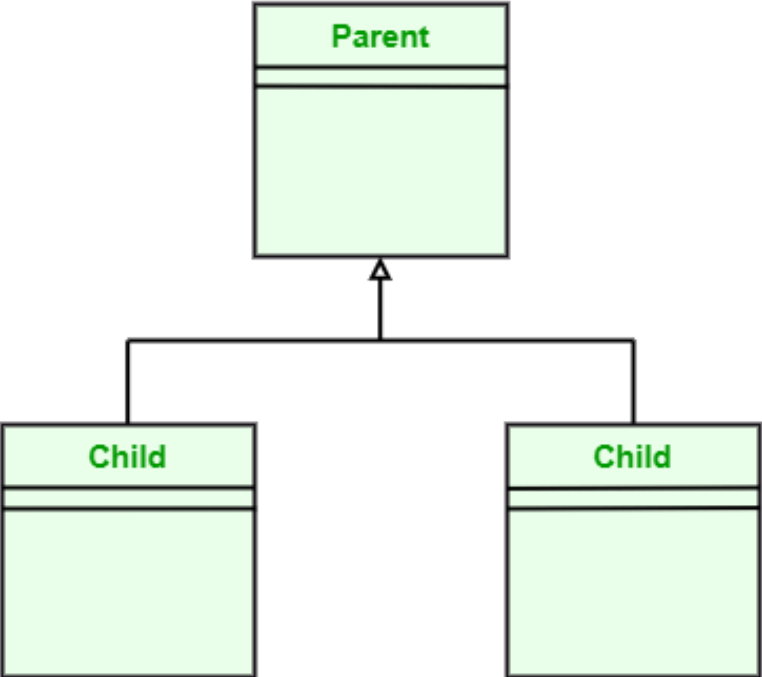
Multiple Inheritance
