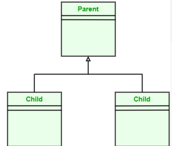
Multiple Inheritance
