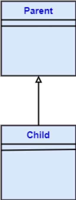
Single Inheritance
