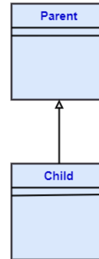
Single Inheritance
